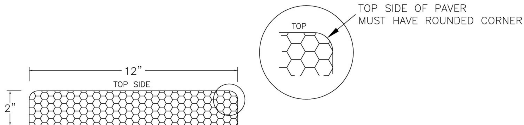
FIGURE 1.1 – PAVER DETAIL
